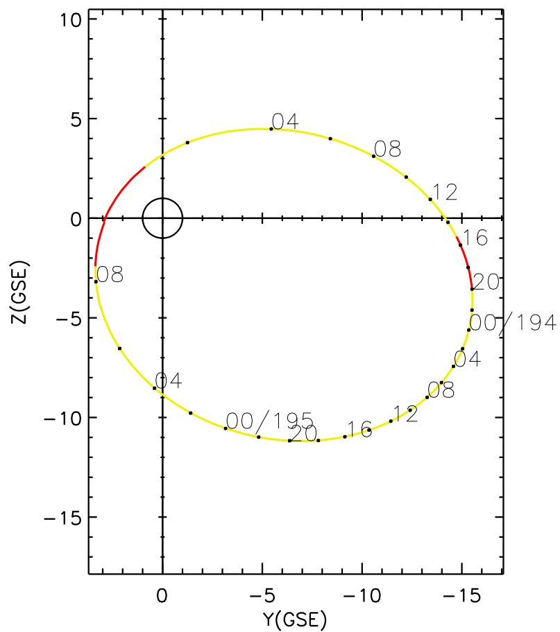
CLUSTER 2 orbit 2007 193 (07/12) 00:05 UT to 2007 195 (07/14) 09:10 UT
