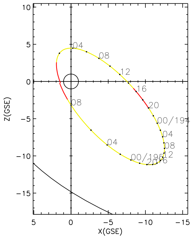
CLUSTER 2 orbit 2007 193 (07/12) 00:05 UT to 2007 195 (07/14) 09:10 UT
