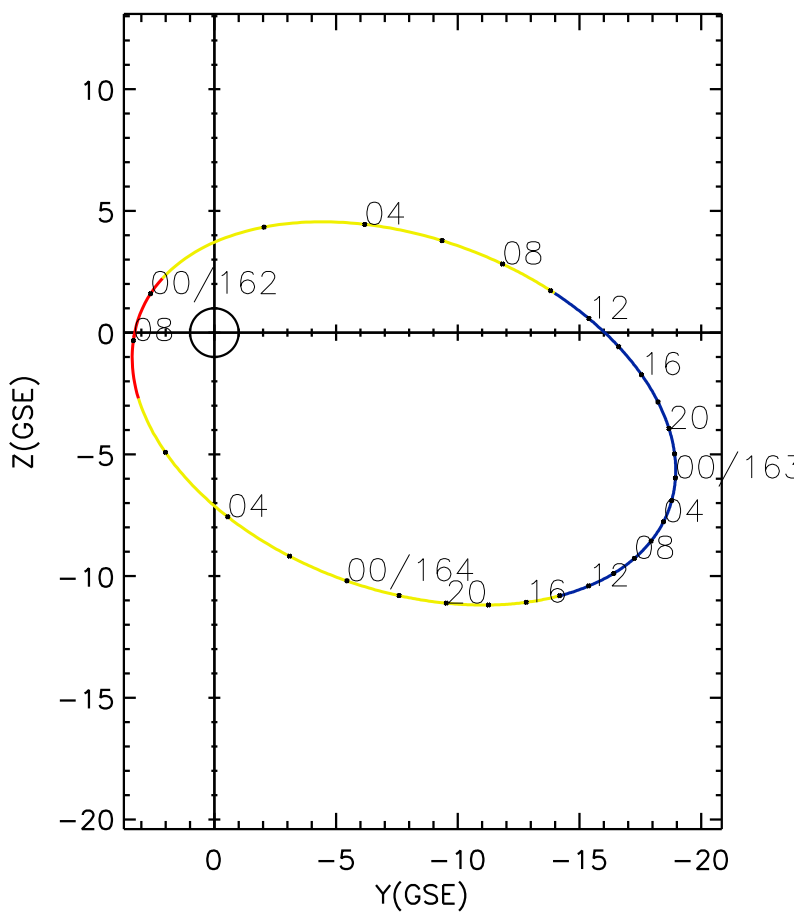
CLUSTER 2 orbit 2007 161 (06/10) 23:21 UT to 2007 164 (06/13) 08:06 UT
