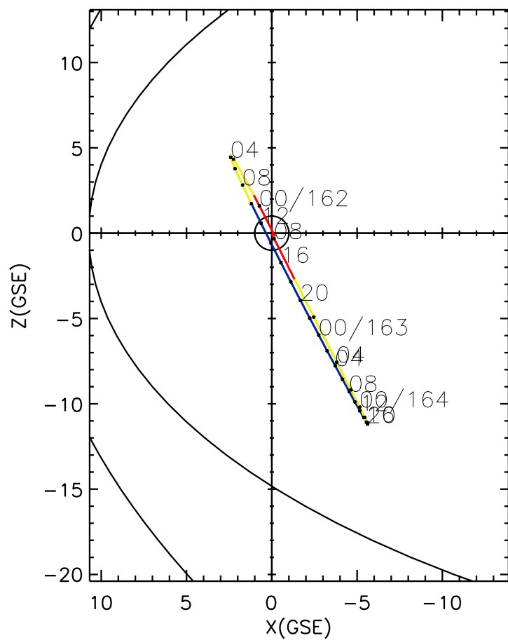
CLUSTER 2 orbit 2007 161 (06/10) 23:21 UT to 2007 164 (06/13) 08:06 UT
