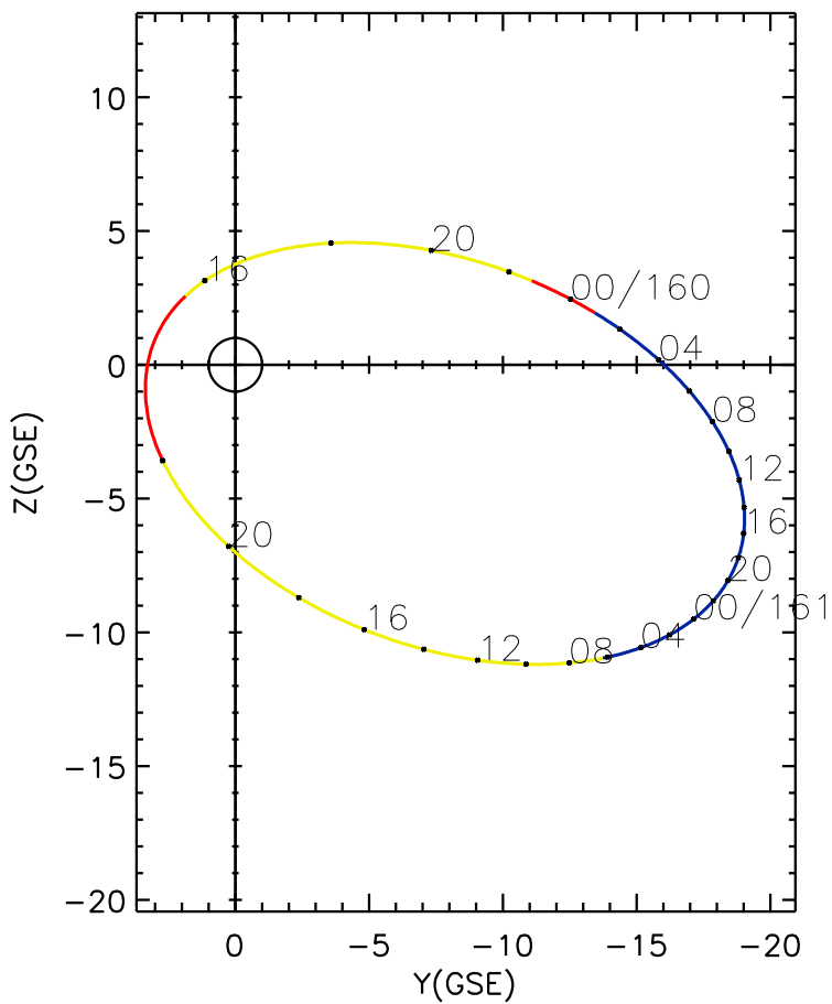
CLUSTER 2 orbit 2007 159 (06/08) 14:36 UT to 2007 161 (06/10) 23:21 UT
