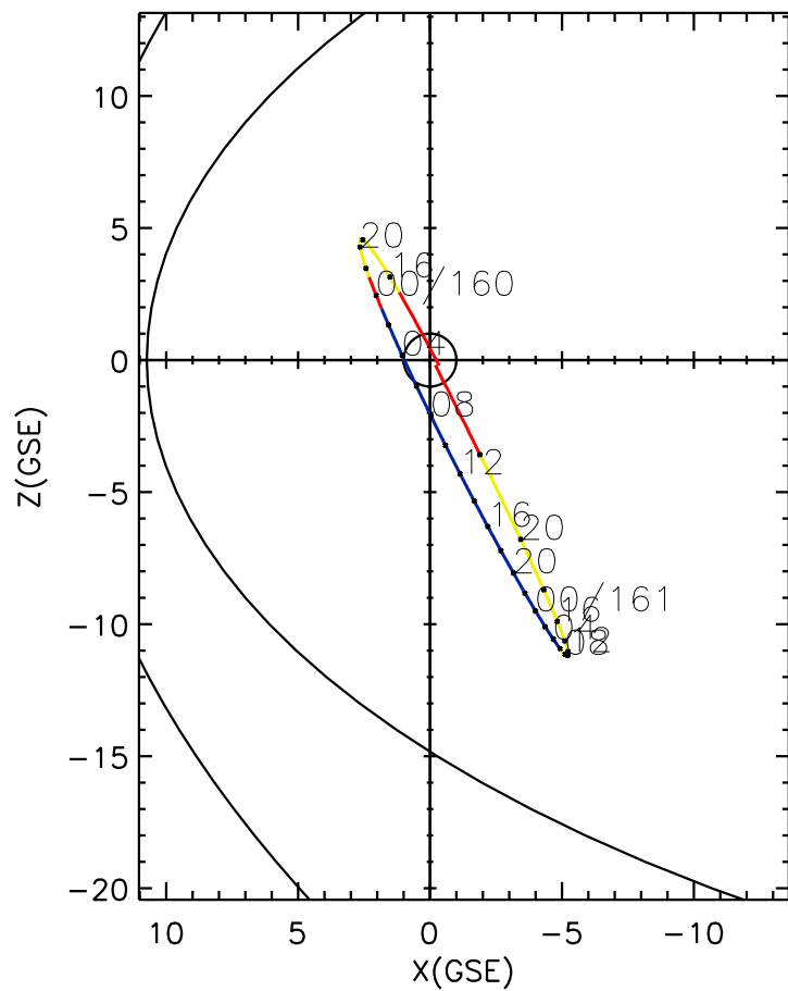
CLUSTER 2 orbit 2007 159 (06/08) 14:36 UT to 2007 161 (06/10) 23:21 UT
