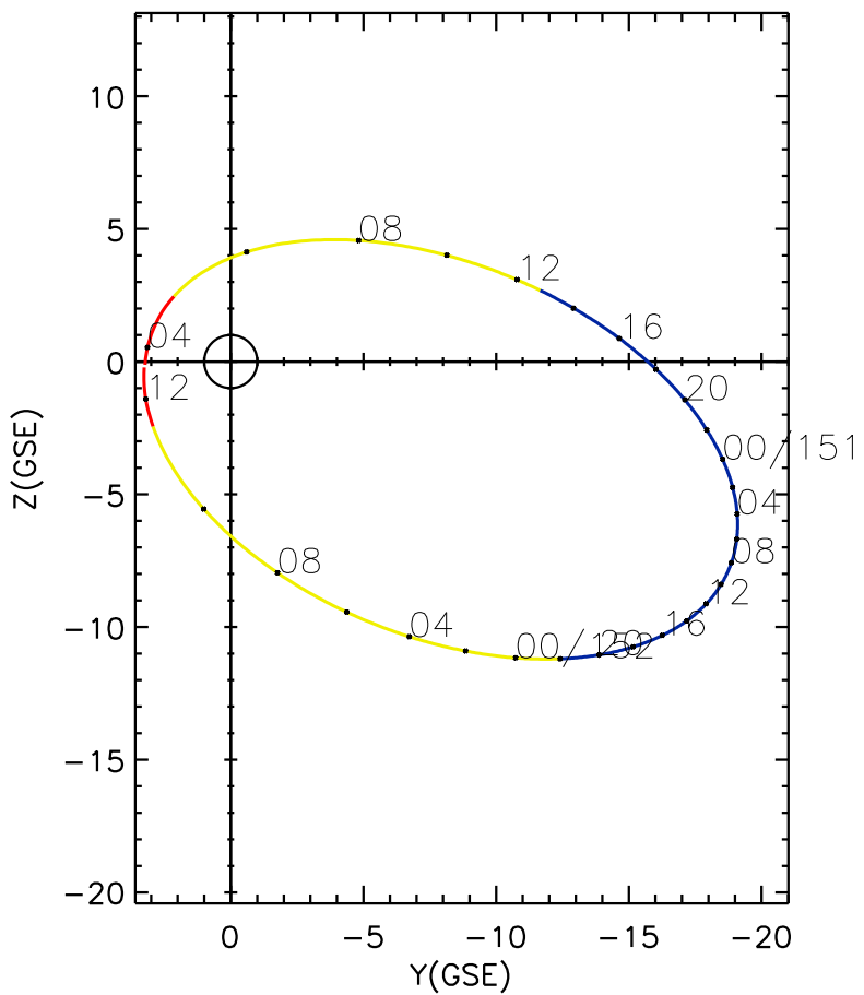
CLUSTER 2 orbit 2007 150 (05/30) 03:46 UT to 2007 152 (06/01) 12:26 UT
