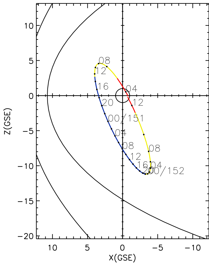
CLUSTER 2 orbit 2007 150 (05/30) 03:46 UT to 2007 152 (06/01) 12:26 UT
