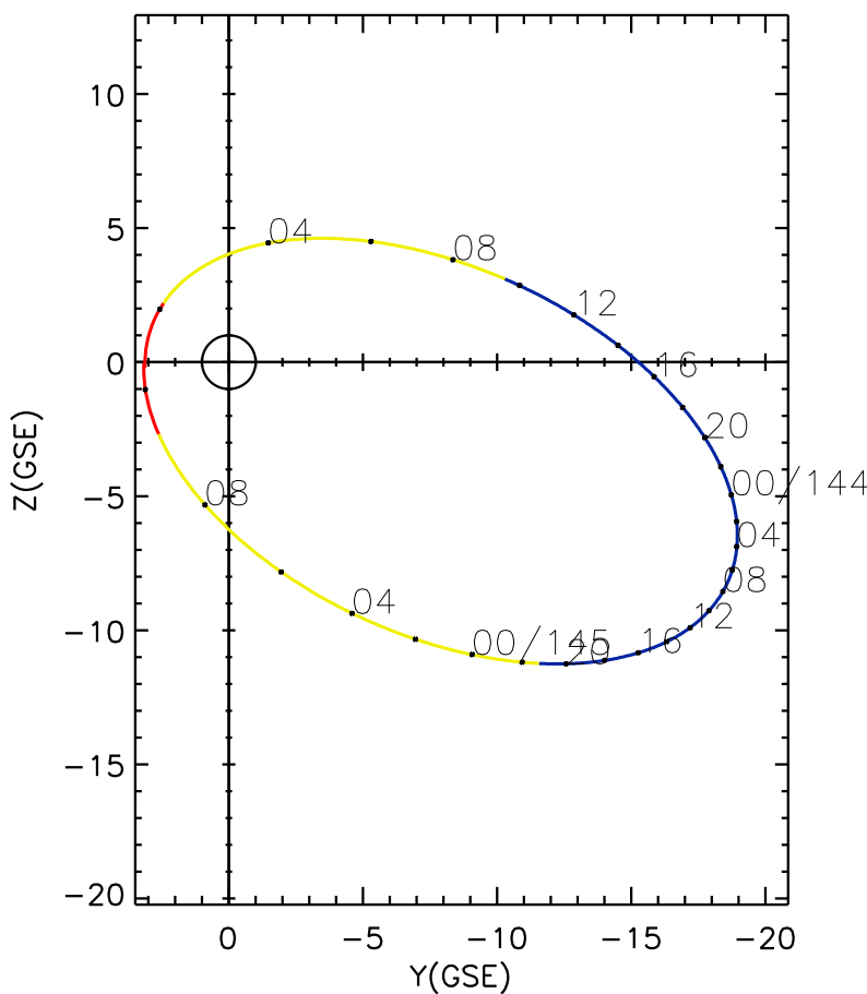
CLUSTER 2 orbit 2007 143 (05/23) 01:11 UT to 2007 145 (05/25) 10:21 UT
