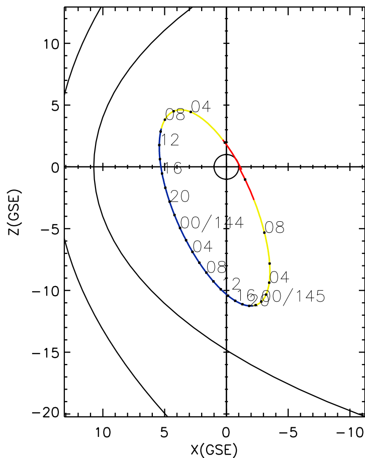
CLUSTER 2 orbit 2007 143 (05/23) 01:11 UT to 2007 145 (05/25) 10:21 UT
