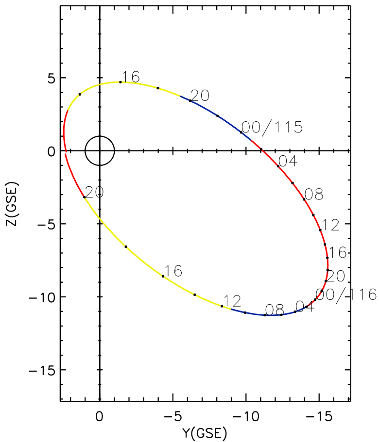
CLUSTER 2 orbit 2007 114 (04/24) 12:06 UT to 2007 116 (04/26) 21:11 UT
