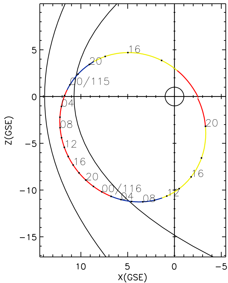
CLUSTER 2 orbit 2007 114 (04/24) 12:06 UT to 2007 116 (04/26) 21:11 UT
