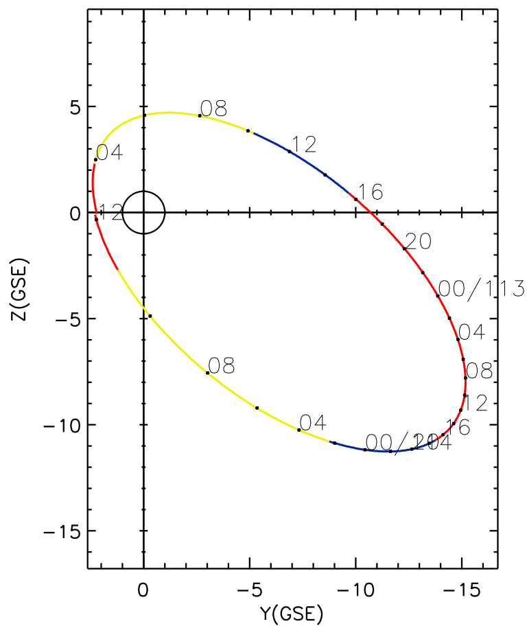
CLUSTER 2 orbit 2007 112 (04/22) 03:00 UT to 2007 114 (04/24) 12:05 UT
