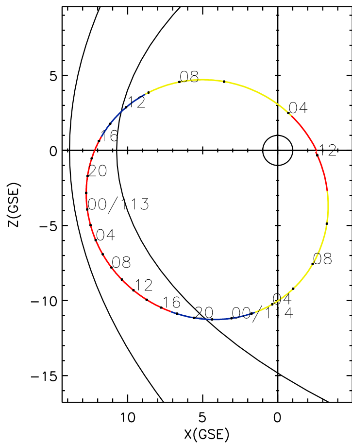
CLUSTER 2 orbit 2007 112 (04/22) 03:00 UT to 2007 114 (04/24) 12:05 UT
