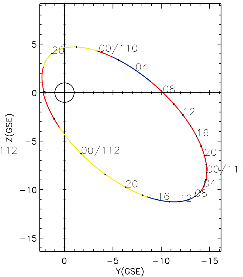
CLUSTER 2 orbit 2007 109 (04/19) 17:56 UT to 2007 112 (04/22) 03:01 UT
