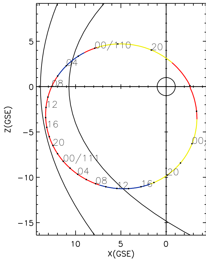
CLUSTER 2 orbit 2007 109 (04/19) 17:56 UT to 2007 112 (04/22) 03:01 UT
