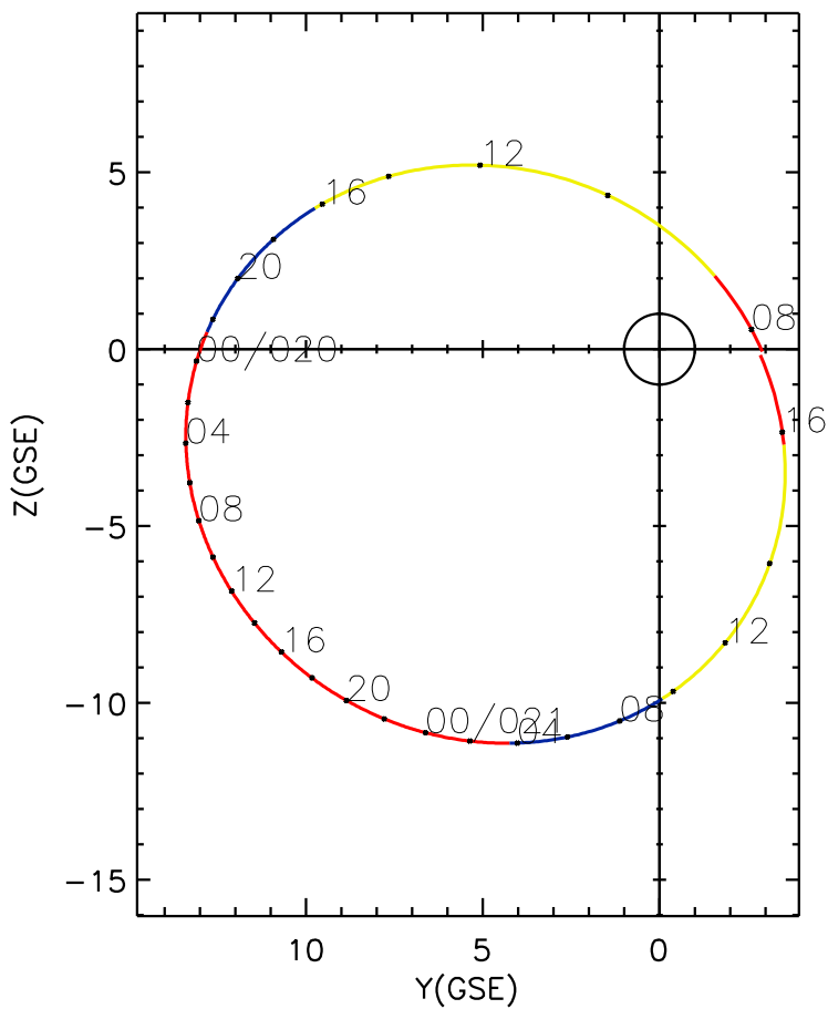
CLUSTER 2 orbit 2007 019 (01/19) 07:46 UT to 2007 021 (01/21) 16:51 UT
