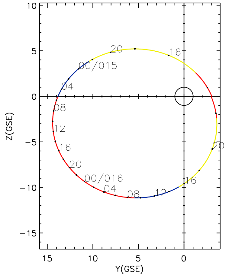
CLUSTER 2 orbit 2007 014 (01/14) 13:36 UT to 2007 016 (01/16) 22:41 UT
