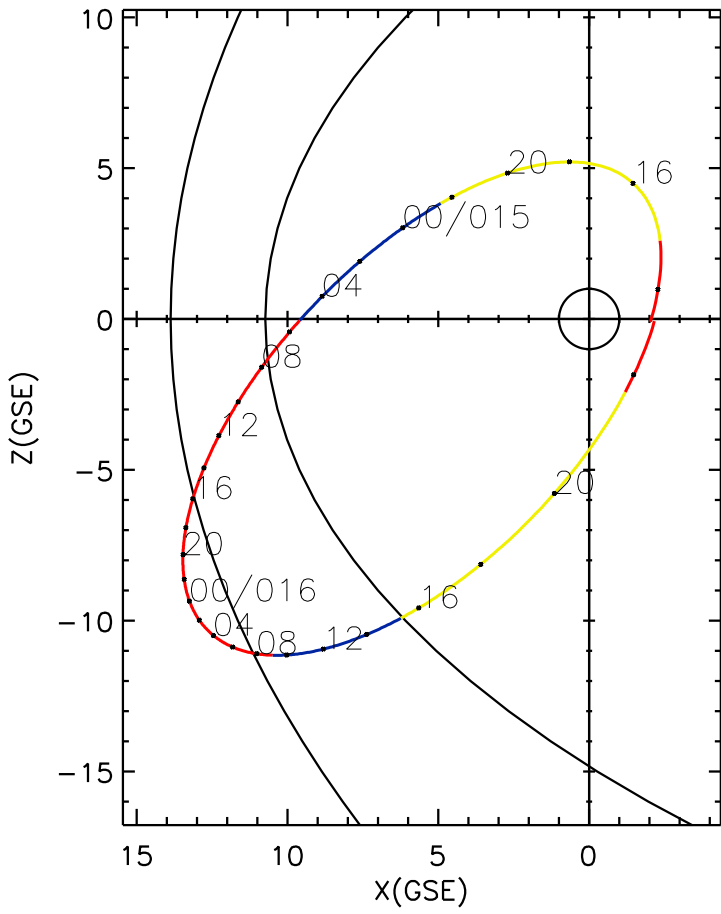
CLUSTER 2 orbit 2007 014 (01/14) 13:36 UT to 2007 016 (01/16) 22:41 UT
