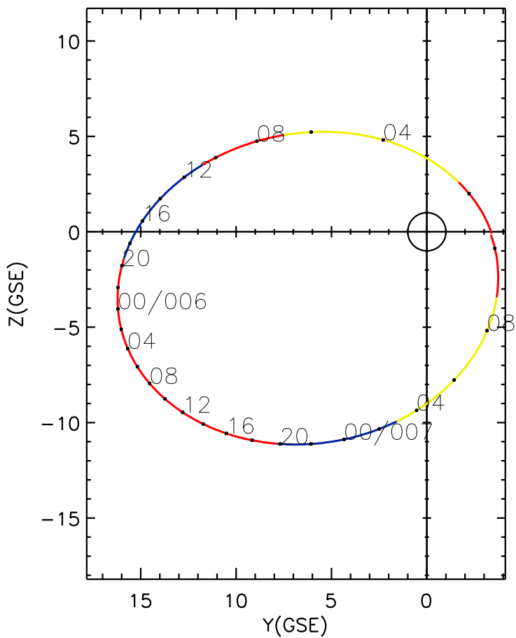
CLUSTER 2 orbit 2007 005 (01/05) 01:11 UT to 2007 007 (01/07) 10:16 UT
