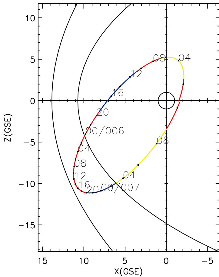
CLUSTER 2 orbit 2007 005 (01/05) 01:11 UT to 2007 007 (01/07) 10:16 UT
