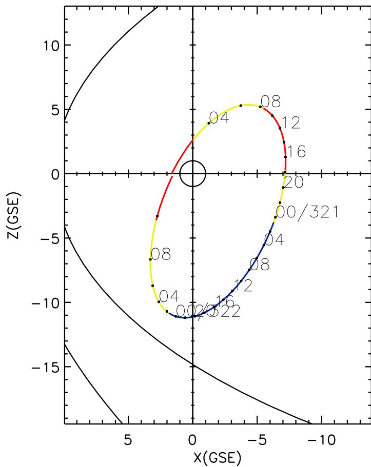
CLUSTER 2 orbit 2006 320 (11/16) 02:11 UT to 2006 322 (11/18) 11:16 UT
