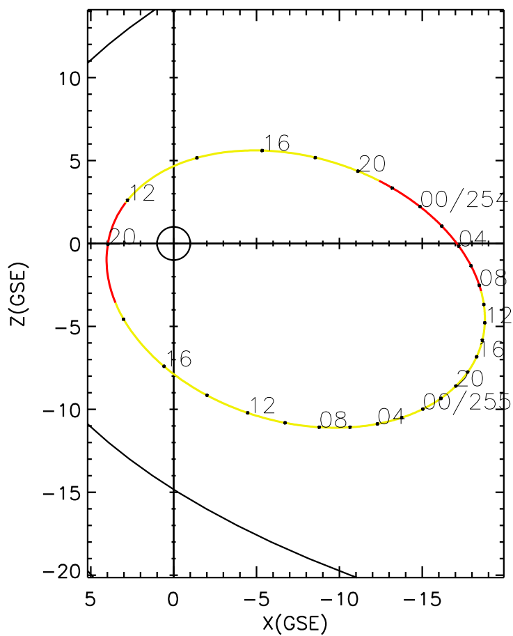
CLUSTER 2 orbit 2006 253 (09/10) 10:51 UT to 2006 255 (09/12) 20:01 UT
