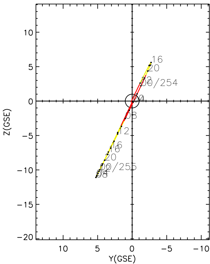
CLUSTER 2 orbit 2006 253 (09/10) 10:51 UT to 2006 255 (09/12) 20:01 UT
