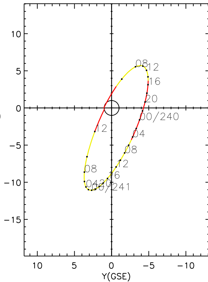
CLUSTER 2 orbit 2006 239 (08/27) 04:11 UT to 2006 241 (08/29) 13:16 UT
