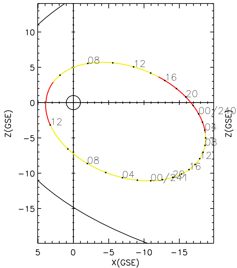
CLUSTER 2 orbit 2006 239 (08/27) 04:11 UT to 2006 241 (08/29) 13:16 UT
