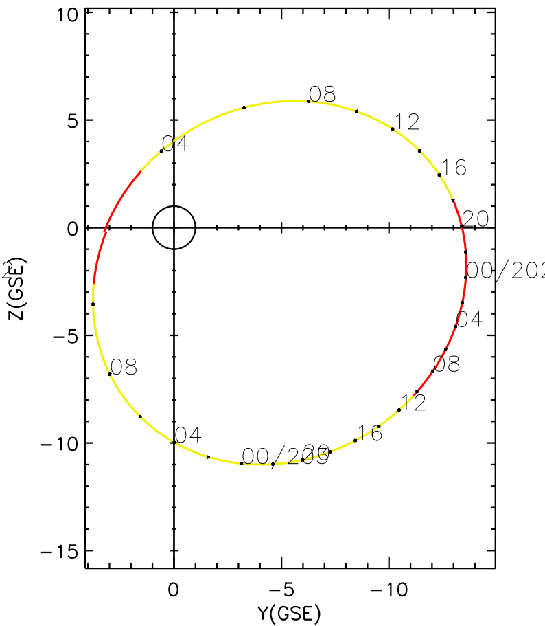
CLUSTER 2 orbit 2006 201 (07/20) 02:21 UT to 2006 203 (07/22) 11:26 UT
