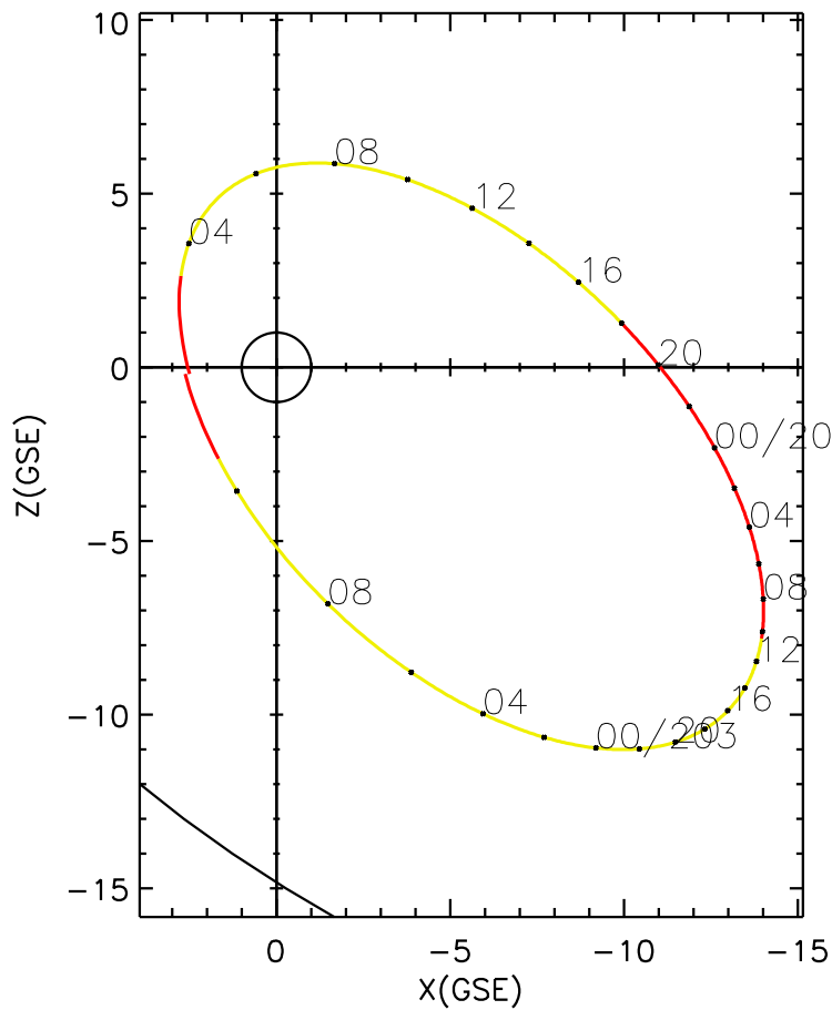
CLUSTER 2 orbit 2006 201 (07/20) 02:21 UT to 2006 203 (07/22) 11:26 UT
