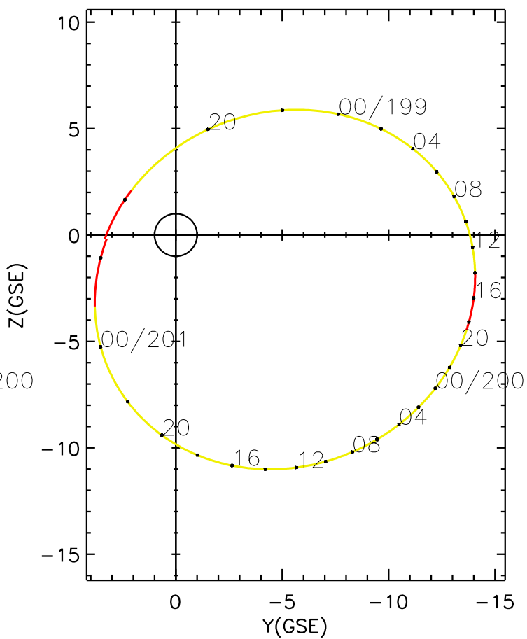
CLUSTER 2 orbit 2006 198 (07/17) 17:16 UT to 2006 201 (07/20) 02:21 UT
