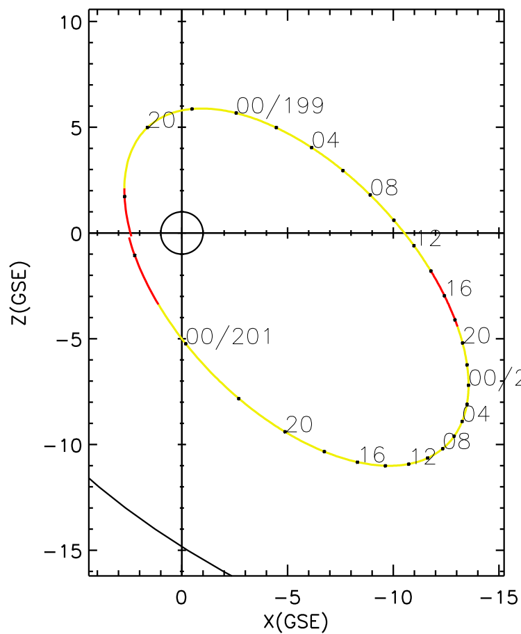
CLUSTER 2 orbit 2006 198 (07/17) 17:15 UT to 2006 201 (07/20) 02:20 UT
