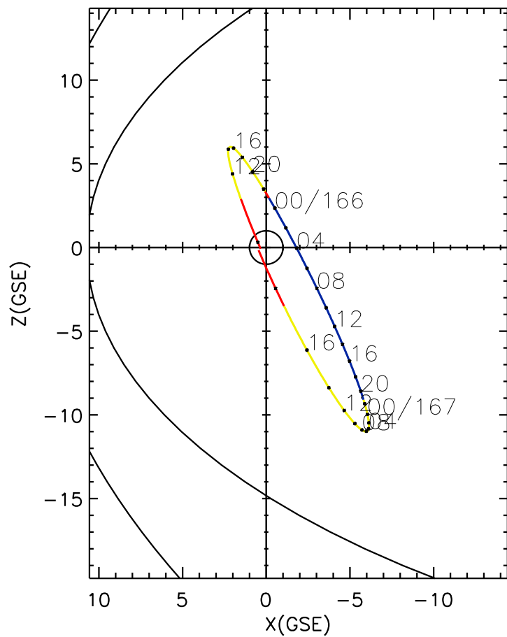
CLUSTER 2 orbit 2006 165 (06/14) 09:51 UT to 2006 167 (06/16) 18:56 UT
