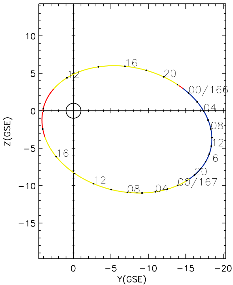
CLUSTER 2 orbit 2006 165 (06/14) 09:51 UT to 2006 167 (06/16) 18:56 UT
