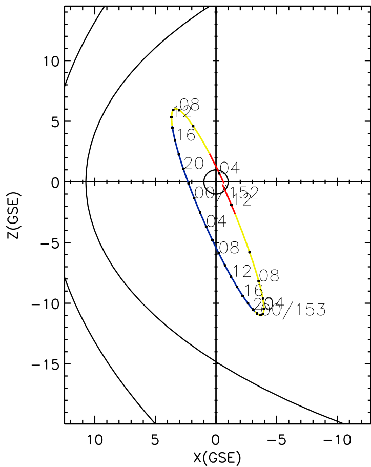
CLUSTER 2 orbit 2006 151 (05/31) 03:41 UT to 2006 153 (06/02) 12:41 UT
