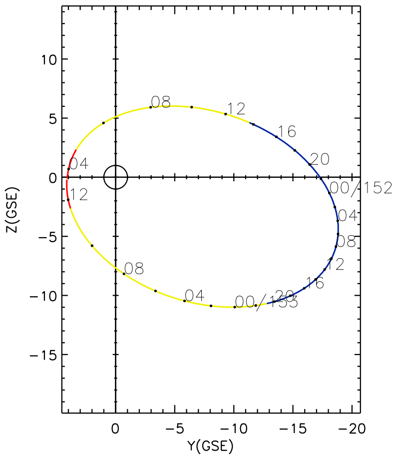
CLUSTER 2 orbit 2006 151 (05/31) 03:41 UT to 2006 153 (06/02) 12:41 UT
