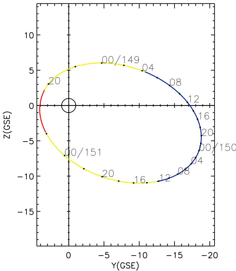
CLUSTER 2 orbit 2006 148 (05/28) 18:41 UT to 2006 151 (05/31) 03:41 UT
