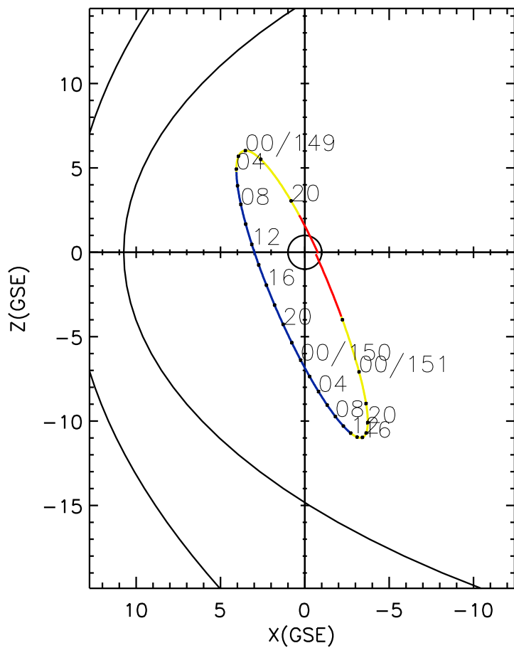
CLUSTER 2 orbit 2006 148 (05/28) 18:41 UT to 2006 151 (05/31) 03:41 UT
