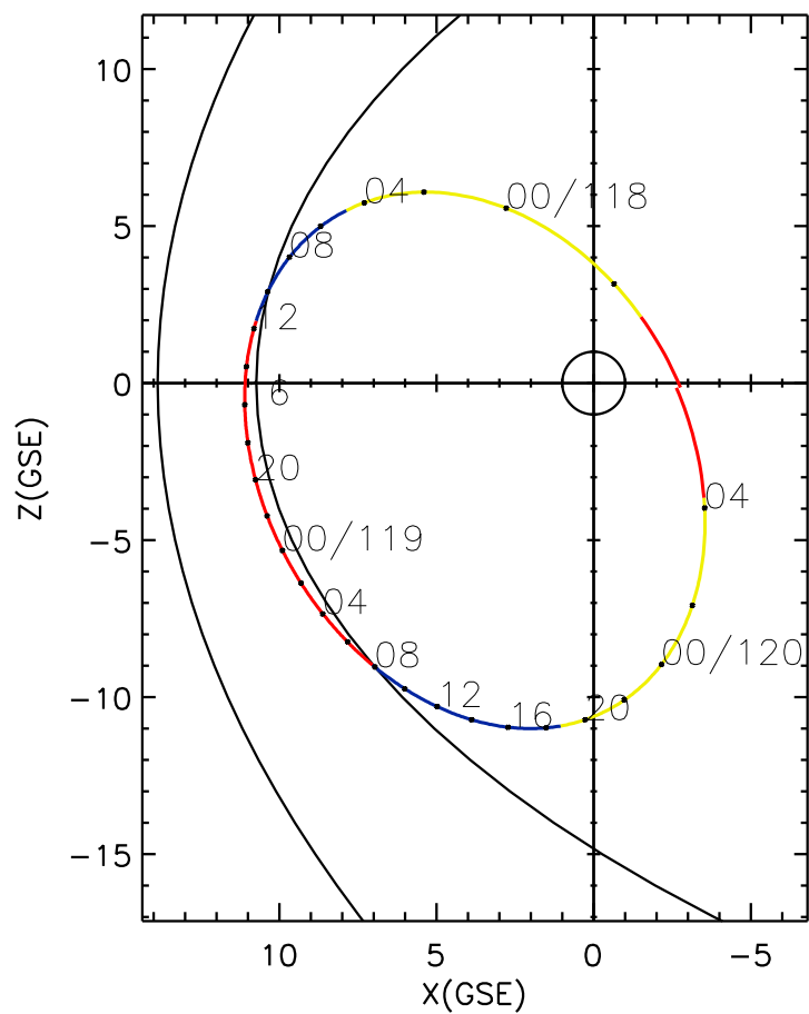
CLUSTER 2 orbit 2006 117 (04/27) 20:35 UT to 2006 120 (04/30) 05:40 UT
