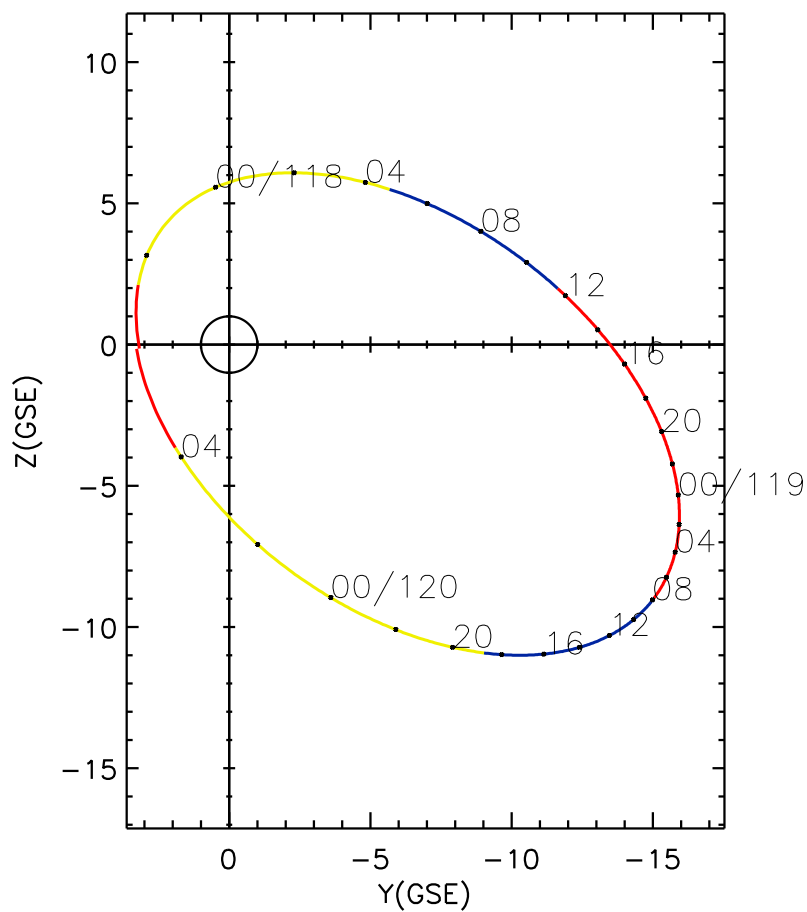
CLUSTER 2 orbit 2006 117 (04/27) 20:35 UT to 2006 120 (04/30) 05:40 UT
