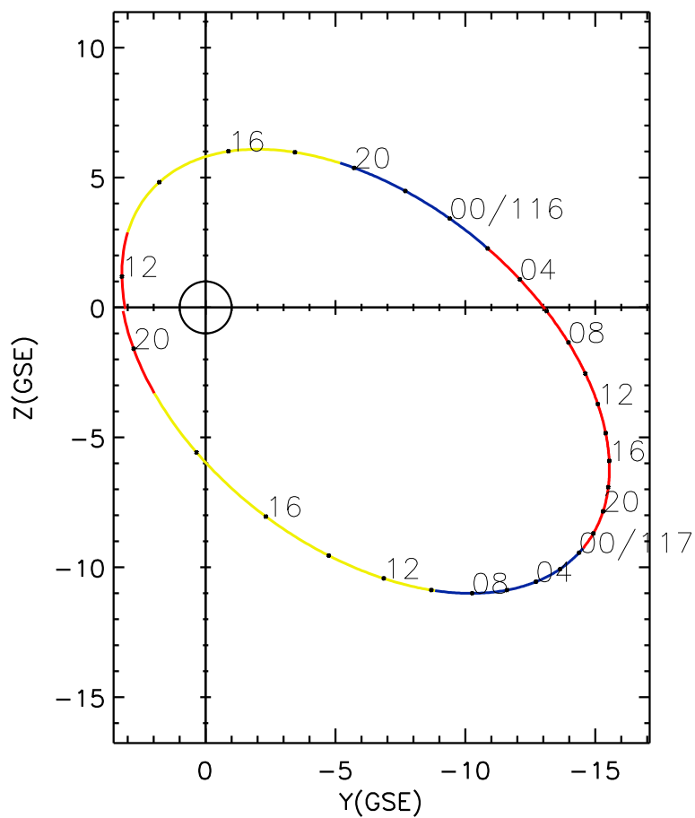
CLUSTER 2 orbit 2006 115 (04/25) 11:30 UT to 2006 117 (04/27) 20:35 UT
