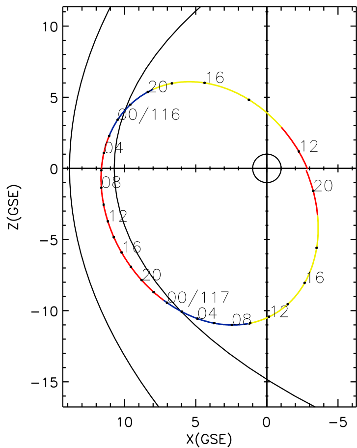
CLUSTER 2 orbit 2006 115 (04/25) 11:30 UT to 2006 117 (04/27) 20:35 UT
