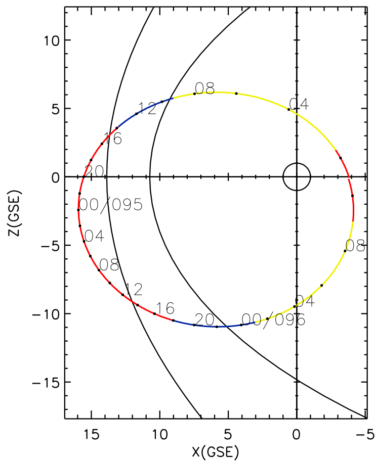
CLUSTER 2 orbit 2006 094 (04/04) 01:25 UT to 2006 096 (04/06) 10:30 UT
