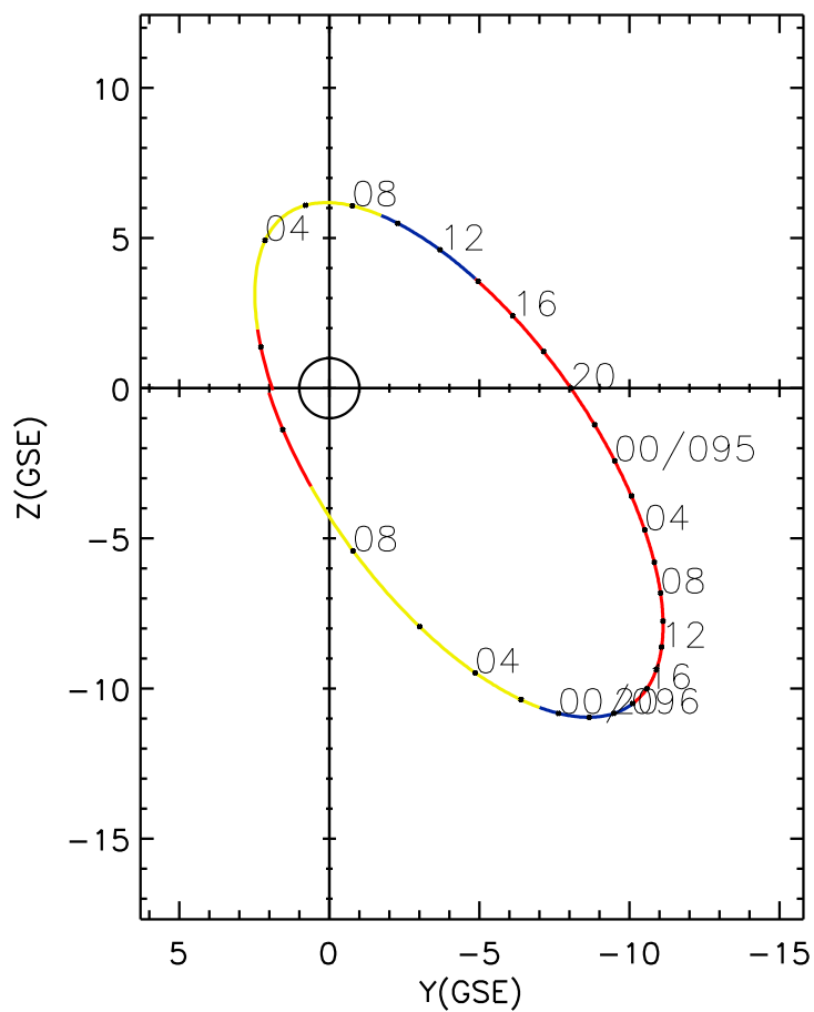
CLUSTER 2 orbit 2006 094 (04/04) 01:25 UT to 2006 096 (04/06) 10:30 UT
