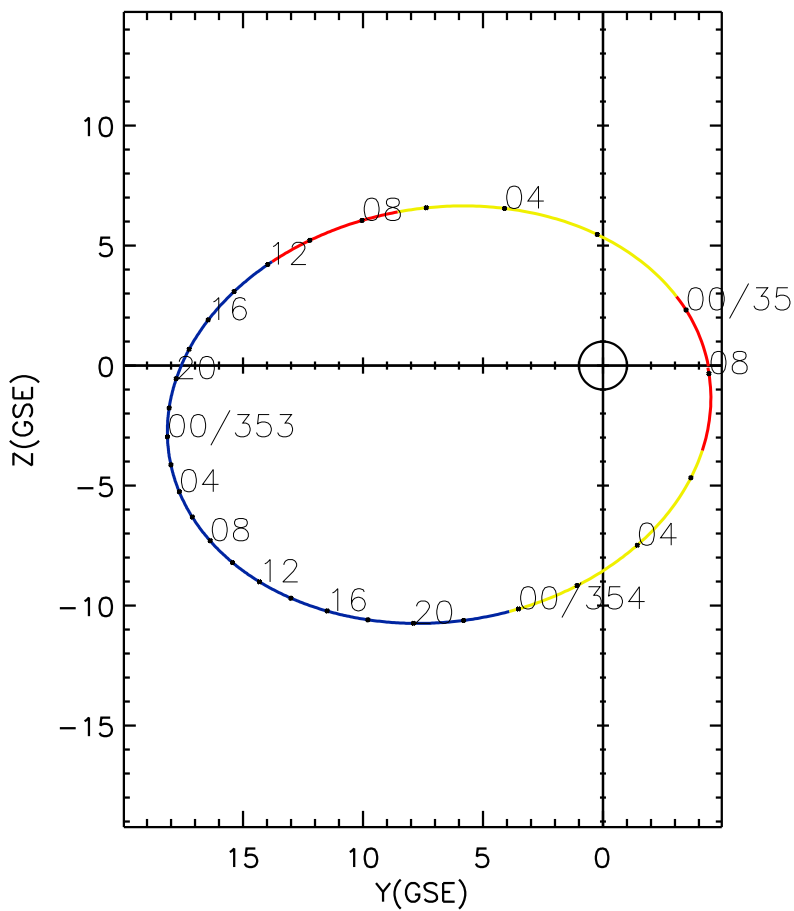
CLUSTER 2 orbit 2005 351 (12/17) 23:01 UT to 2005 354 (12/20) 08:06 UT
