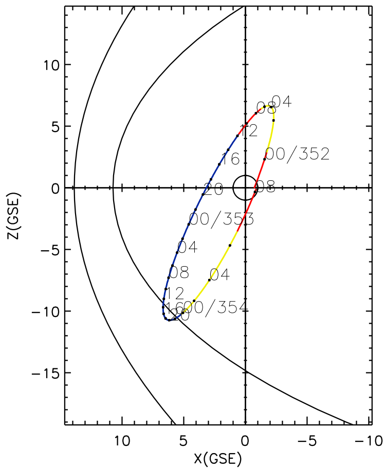
CLUSTER 2 orbit 2005 351 (12/17) 23:01 UT to 2005 354 (12/20) 08:06 UT
