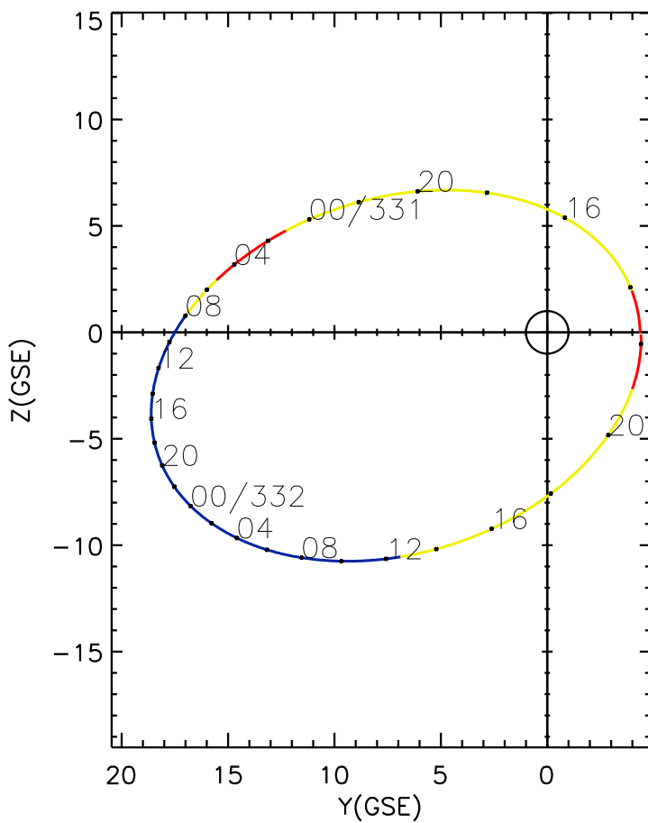
CLUSTER 2 orbit 2005 330 (11/26) 13:06 UT to 2005 332 (11/28) 22:11 UT
