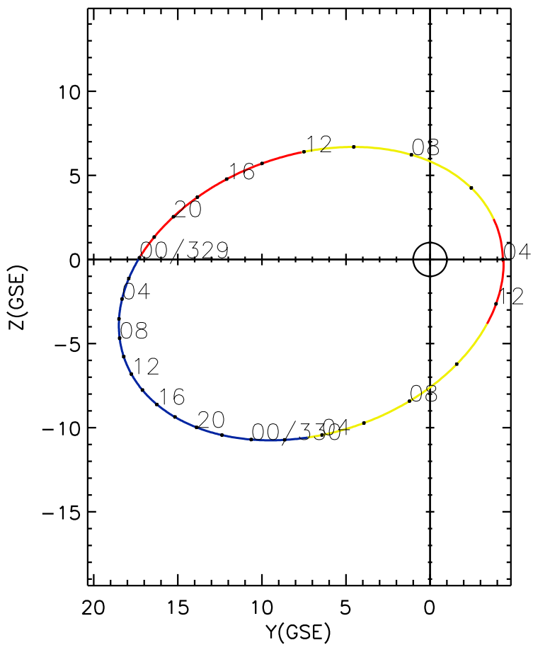
CLUSTER 2 orbit 2005 328 (11/24) 03:56 UT to 2005 330 (11/26) 13:06 UT
