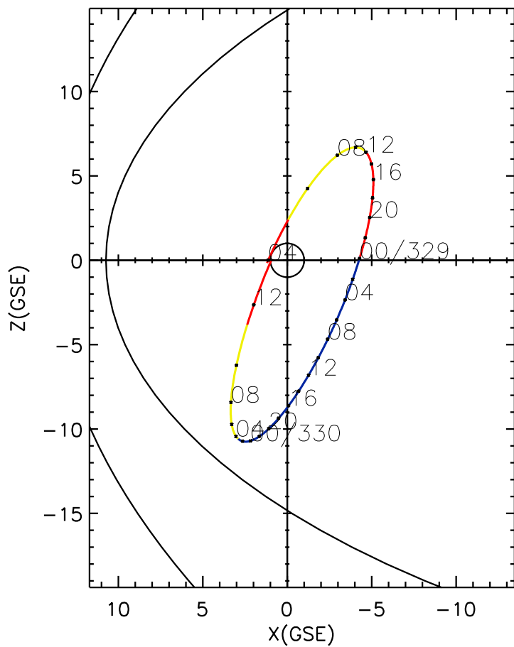
CLUSTER 2 orbit 2005 328 (11/24) 03:56 UT to 2005 330 (11/26) 13:06 UT
