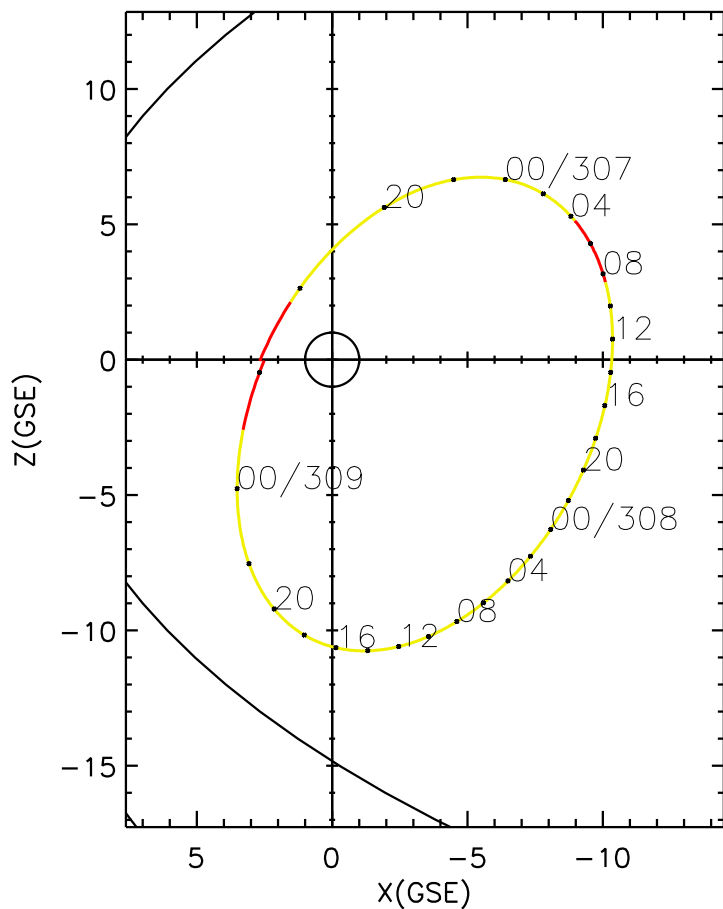
CLUSTER 2 orbit 2005 306 (11/02) 16:51 UT to 2005 309 (11/05) 02:11 UT
