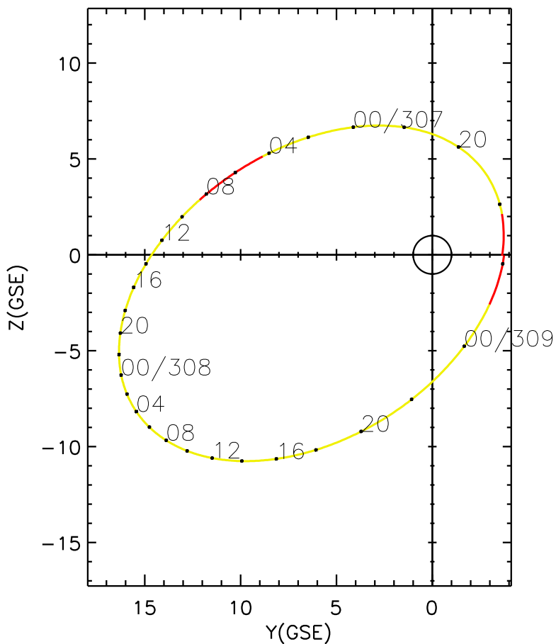
CLUSTER 2 orbit 2005 306 (11/02) 16:51 UT to 2005 309 (11/05) 02:11 UT
