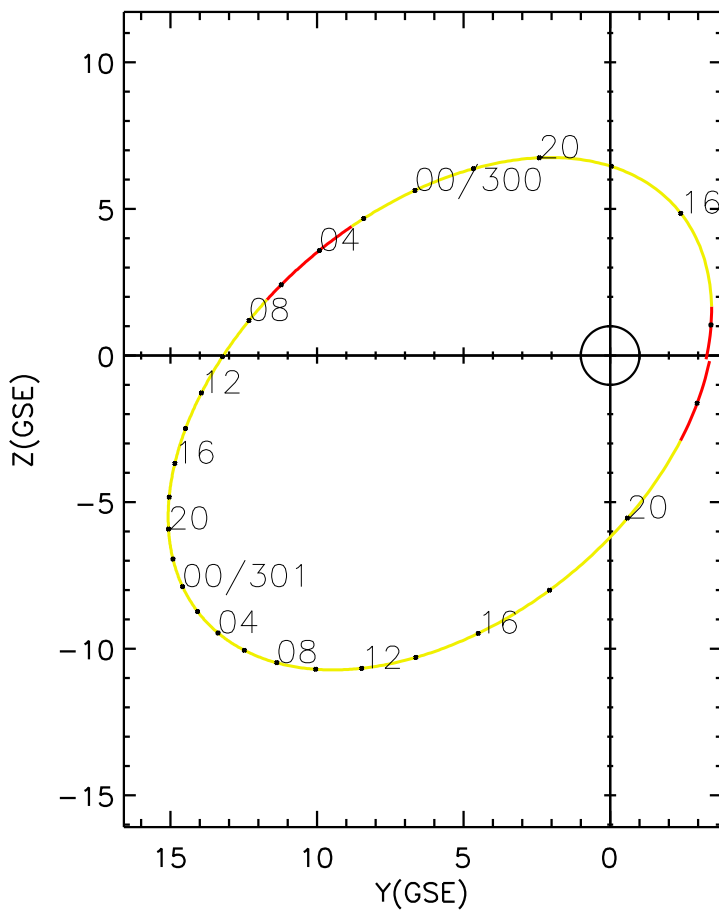
CLUSTER 2 orbit 2005 299 (10/26) 13:31 UT to 2005 301 (10/28) 22:36 UT
