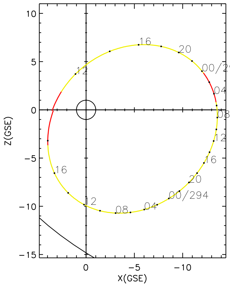
CLUSTER 2 orbit 2005 292 (10/19) 10:16 UT to 2005 294 (10/21) 19:21 UT
