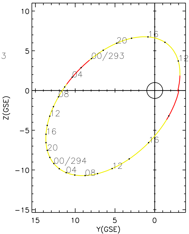
CLUSTER 2 orbit 2005 292 (10/19) 10:16 UT to 2005 294 (10/21) 19:21 UT
