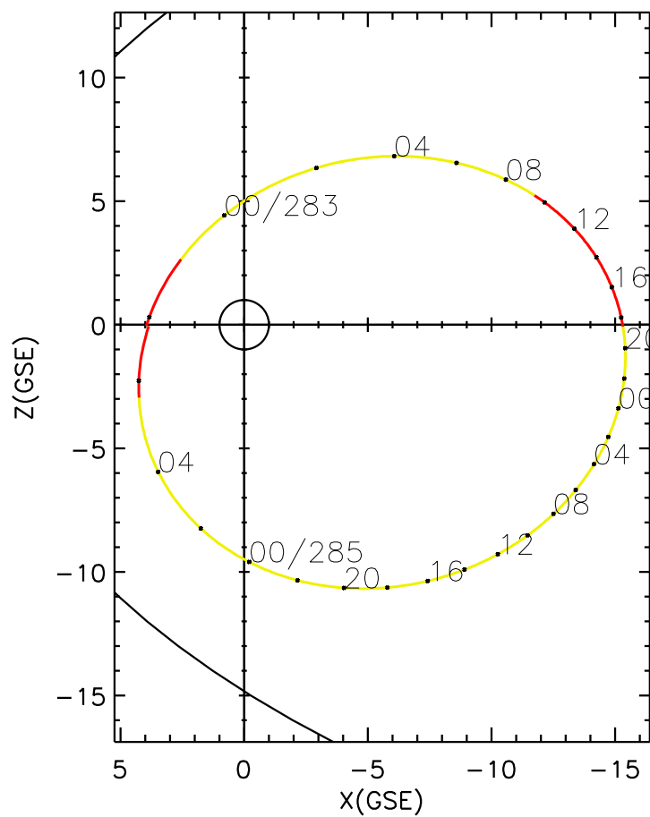
CLUSTER 2 orbit 2005 282 (10/09) 21:51 UT to 2005 285 (10/12) 06:56 UT
