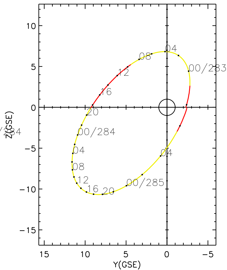
CLUSTER 2 orbit 2005 282 (10/09) 21:51 UT to 2005 285 (10/12) 06:56 UT
