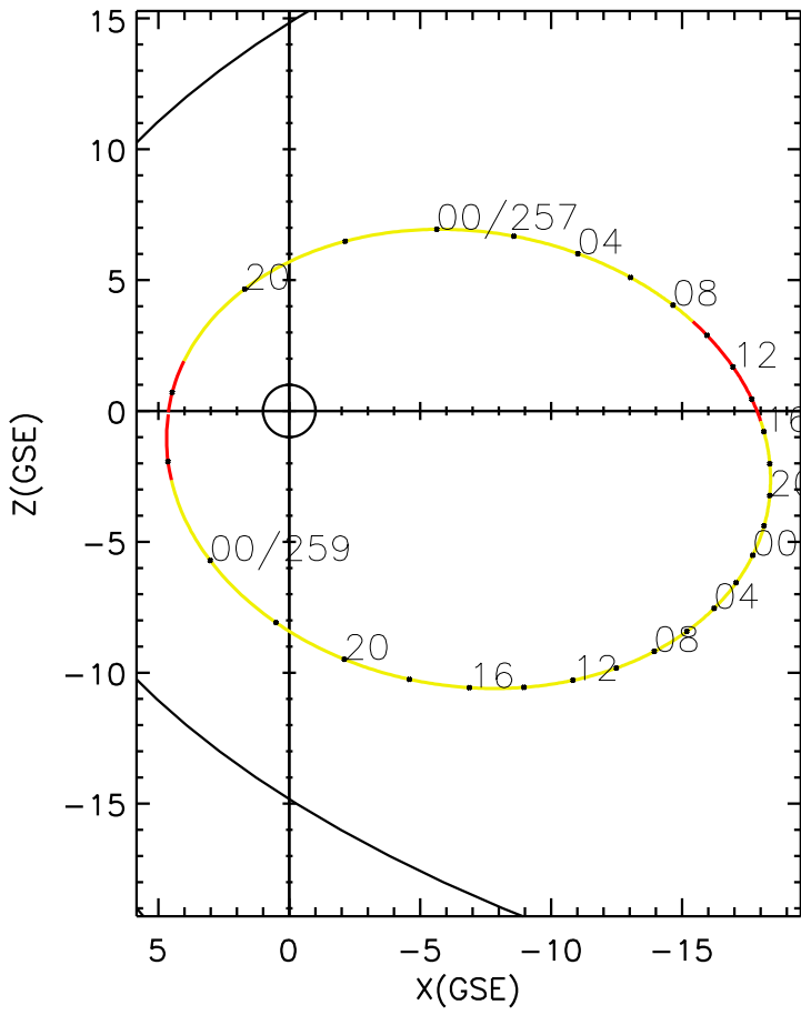
CLUSTER 2 orbit 2005 256 (09/13) 17:41 UT to 2005 259 (09/16) 02:46 UT
