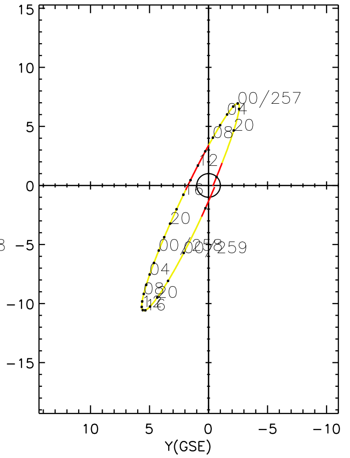
CLUSTER 2 orbit 2005 256 (09/13) 17:41 UT to 2005 259 (09/16) 02:46 UT
