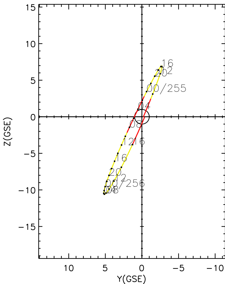
CLUSTER 2 orbit 2005 254 (09/11) 08:36 UT to 2005 256 (09/13) 17:41 UT
