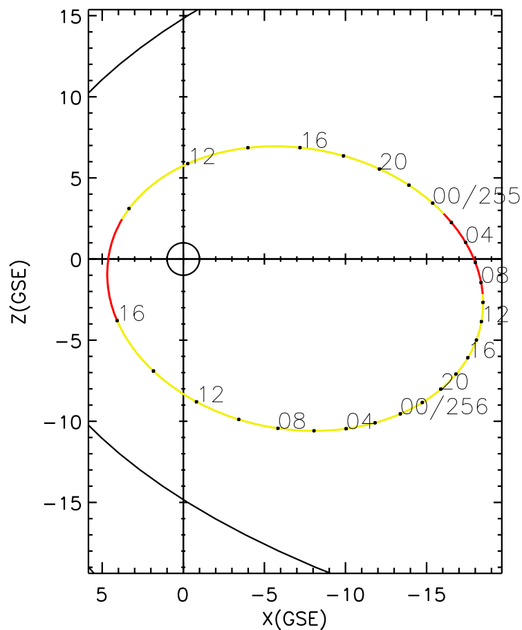
CLUSTER 2 orbit 2005 254 (09/11) 08:36 UT to 2005 256 (09/13) 17:41 UT
