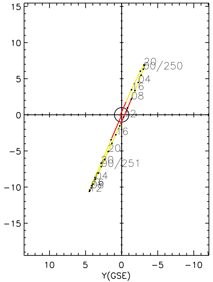
CLUSTER 2 orbit 2005 249 (09/06) 14:21 UT to 2005 251 (09/08) 23:31 UT
