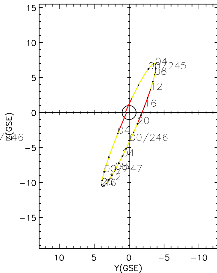
CLUSTER 2 orbit 2005 244 (09/01) 20:11 UT to 2005 247 (09/04) 05:16 UT
