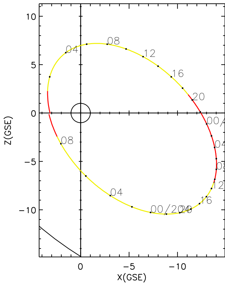
CLUSTER 2 orbit 2005 202 (07/21) 00:16 UT to 2005 204 (07/23) 09:21 UT
