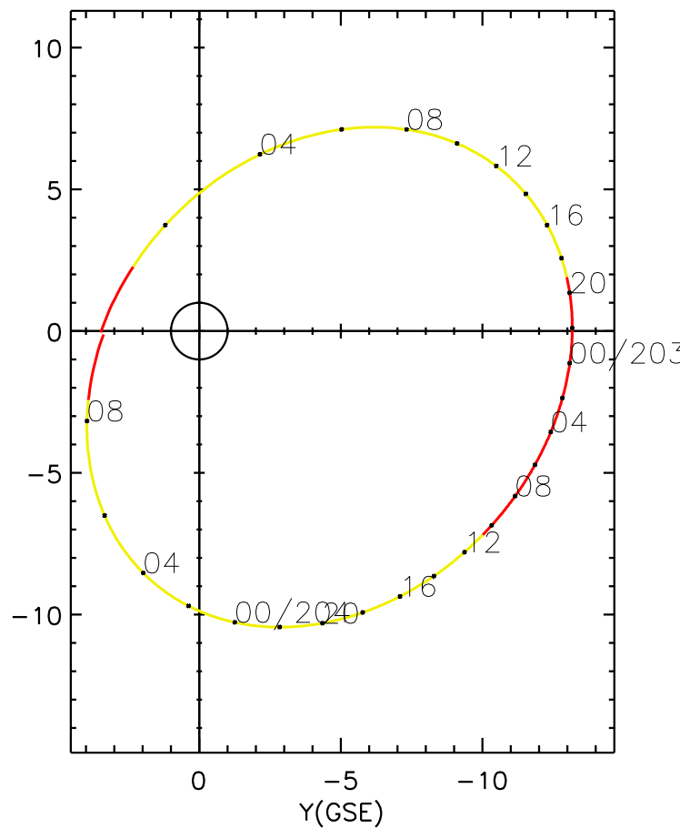
CLUSTER 2 orbit 2005 202 (07/21) 00:16 UT to 2005 204 (07/23) 09:21 UT
