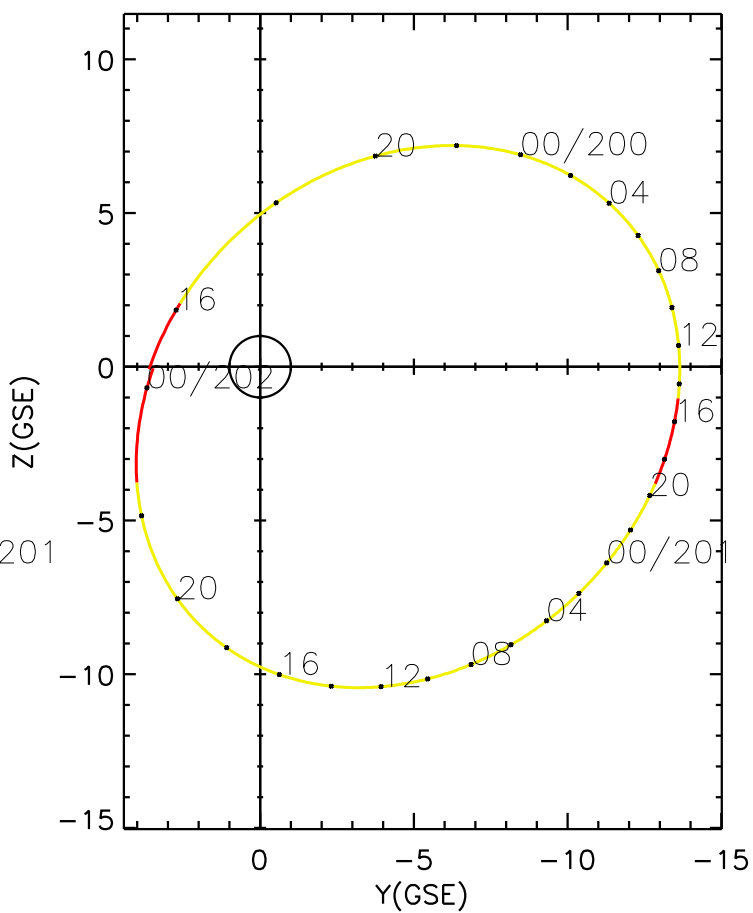
CLUSTER 2 orbit 2005 199 (07/18) 15:11 UT to 2005 202 (07/21) 00:16 UT
