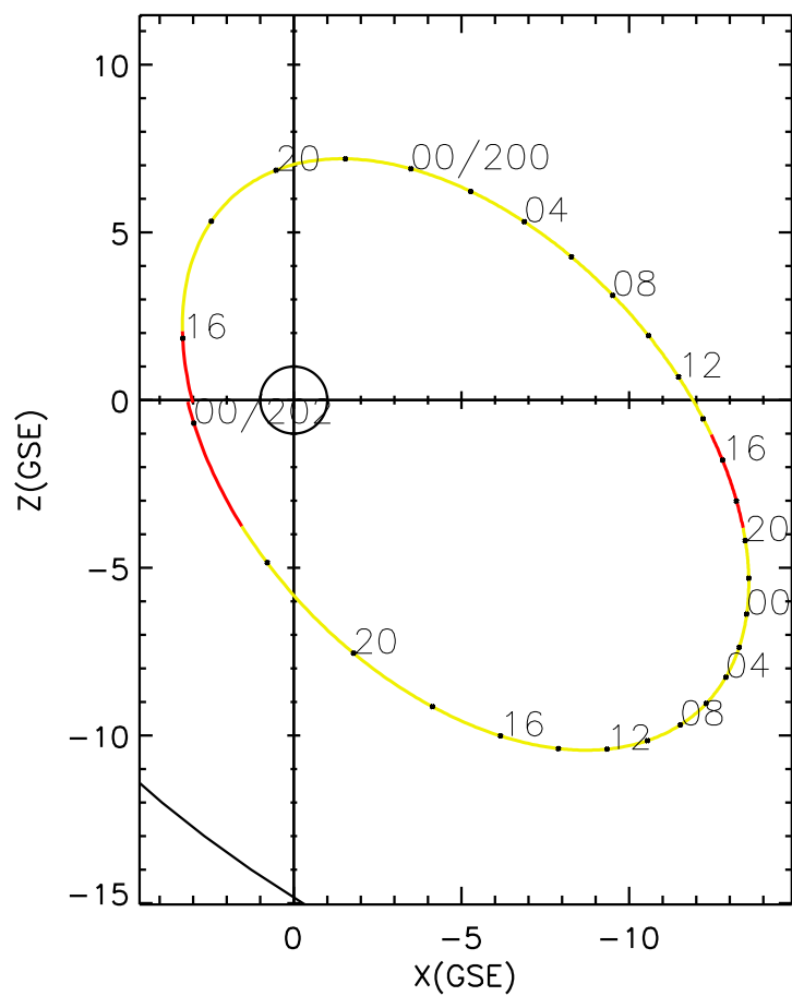
CLUSTER 2 orbit 2005 199 (07/18) 15:11 UT to 2005 202 (07/21) 00:16 UT
