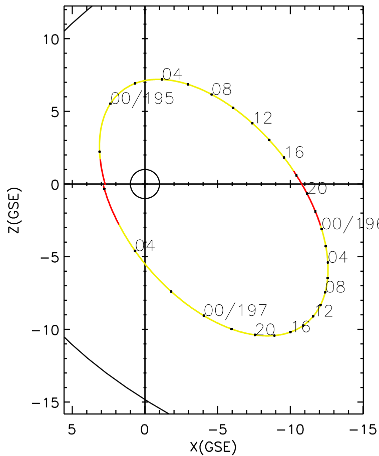
CLUSTER 2 orbit 2005 194 (07/13) 21:01 UT to 2005 197 (07/16) 06:06 UT
