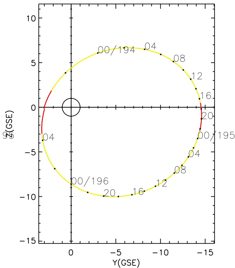
CLUSTER 2 orbit 2005 193 (07/12) 20:20 UT to 2005 196 (07/15) 05:25 UT
