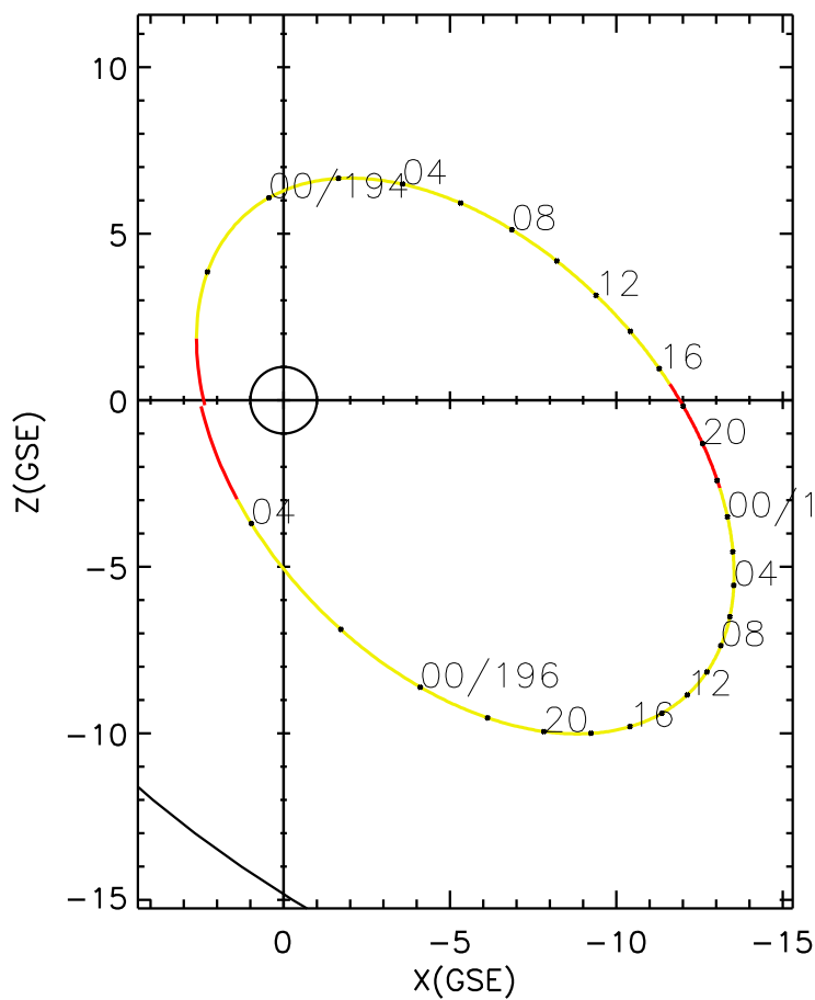
CLUSTER 2 orbit 2005 193 (07/12) 20:20 UT to 2005 196 (07/15) 05:25 UT
