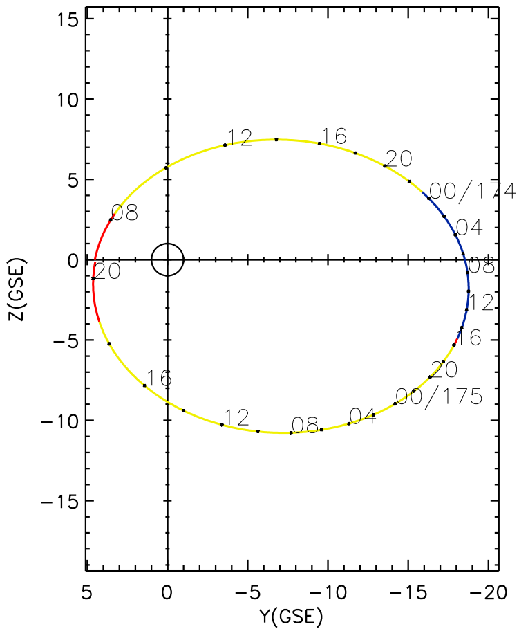
CLUSTER 2 orbit 2005 173 (06/22) 06:56 UT to 2005 175 (06/24) 20:26 UT
