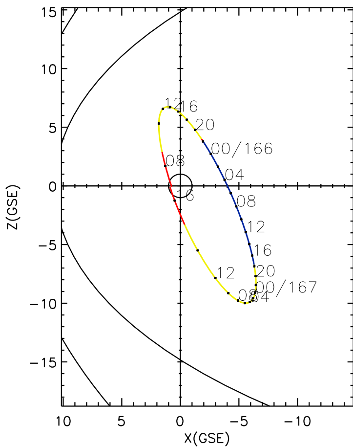
CLUSTER 2 orbit 2005 165 (06/14) 07:20 UT to 2005 167 (06/16) 16:25 UT
