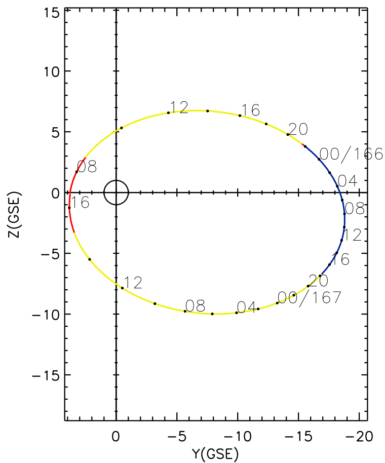
CLUSTER 2 orbit 2005 165 (06/14) 07:20 UT to 2005 167 (06/16) 16:25 UT
