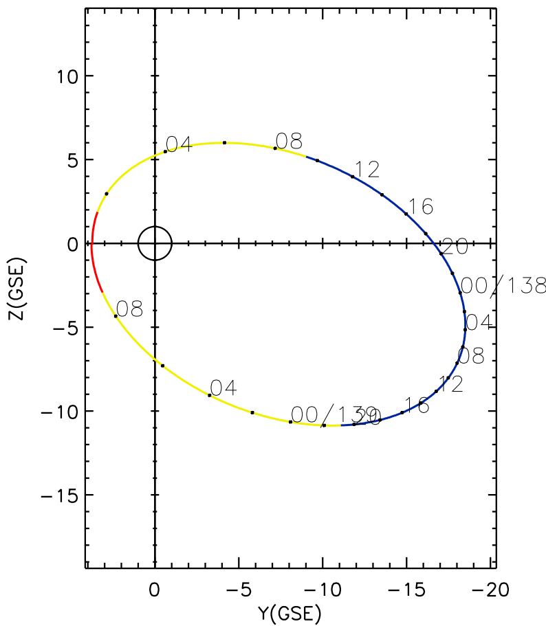
CLUSTER 2 orbit 2005 137 (05/17) 00:46 UT to 2005 139 (05/19) 09:51 UT
