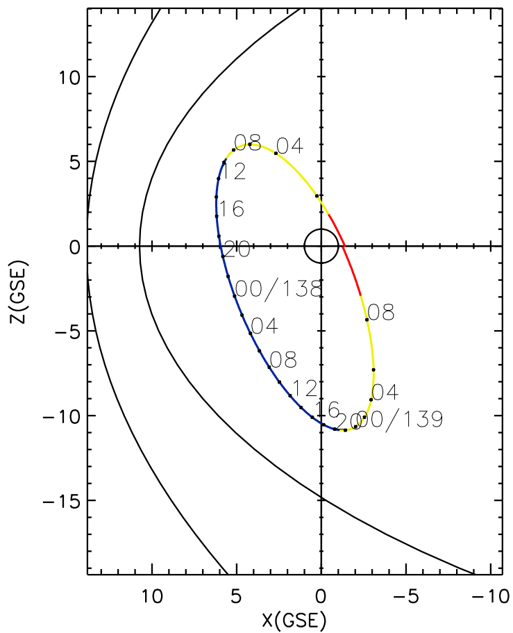
CLUSTER 2 orbit 2005 137 (05/17) 00:46 UT to 2005 139 (05/19) 09:51 UT
