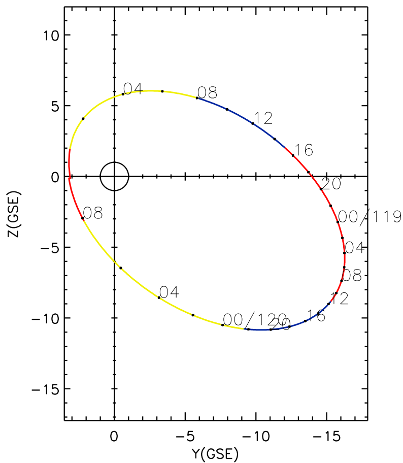
CLUSTER 2 orbit 2005 118 (04/28) 00:05 UT to 2005 120 (04/30) 09:10 UT
