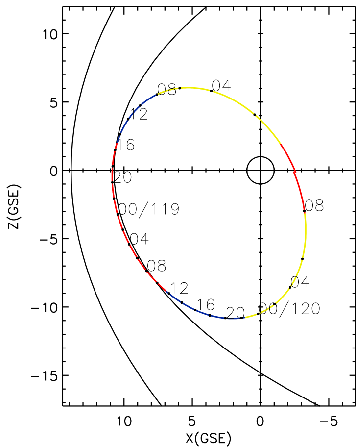
CLUSTER 2 orbit 2005 118 (04/28) 00:05 UT to 2005 120 (04/30) 09:10 UT
