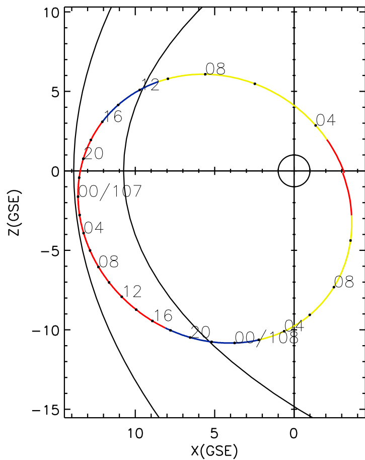
CLUSTER 2 orbit 2005 106 (04/16) 02:46 UT to 2005 108 (04/18) 11:51 UT
