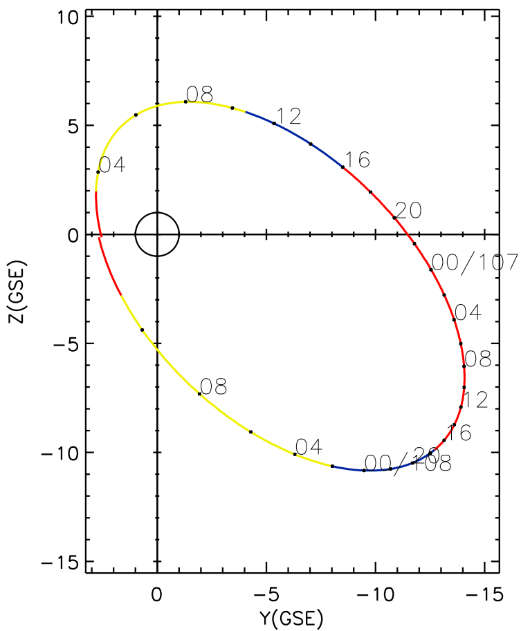
CLUSTER 2 orbit 2005 106 (04/16) 02:46 UT to 2005 108 (04/18) 11:51 UT
