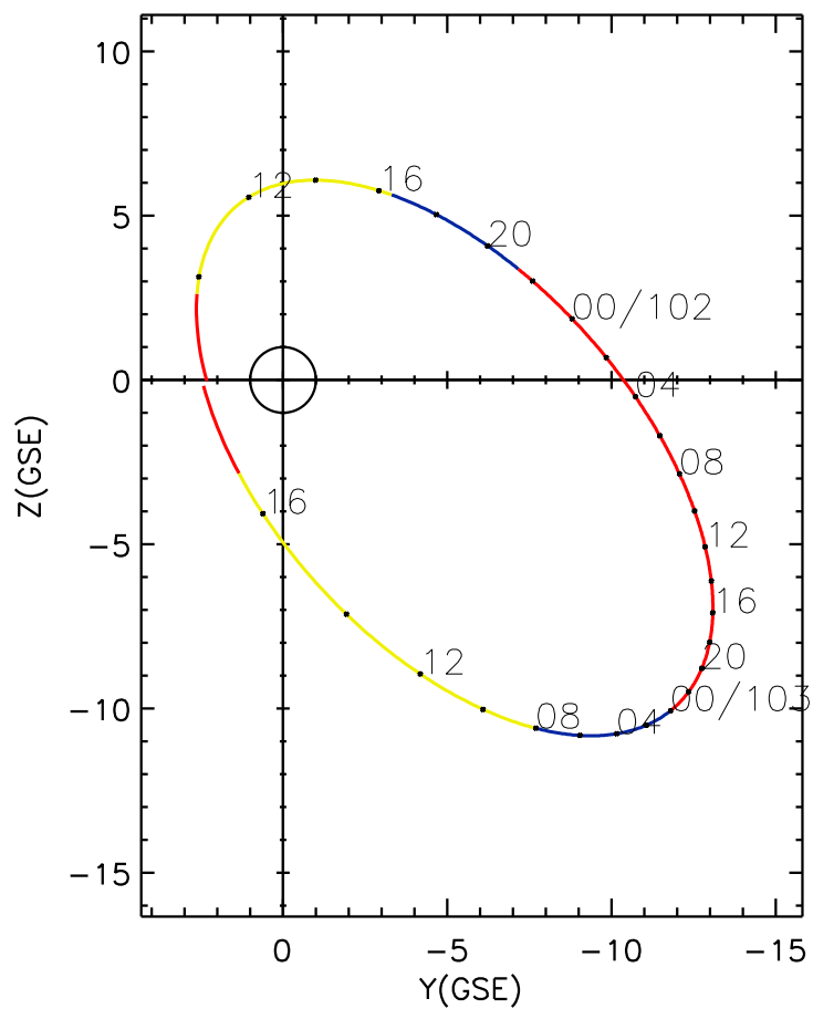
CLUSTER 2 orbit 2005 101 (04/11) 08:40 UT to 2005 103 (04/13) 17:40 UT
