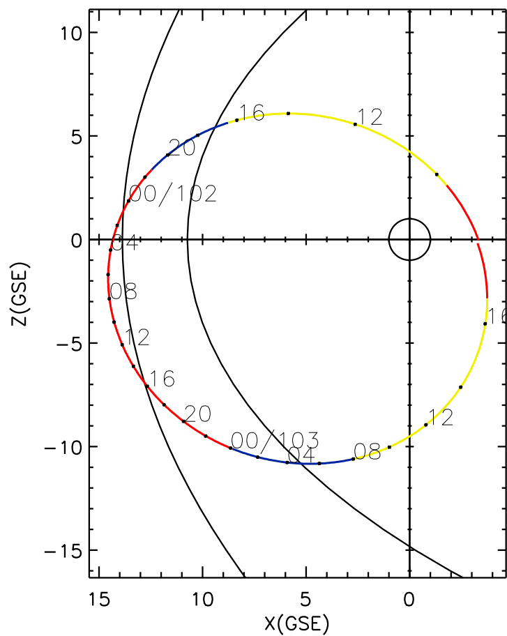
CLUSTER 2 orbit 2005 101 (04/11) 08:40 UT to 2005 103 (04/13) 17:40 UT
