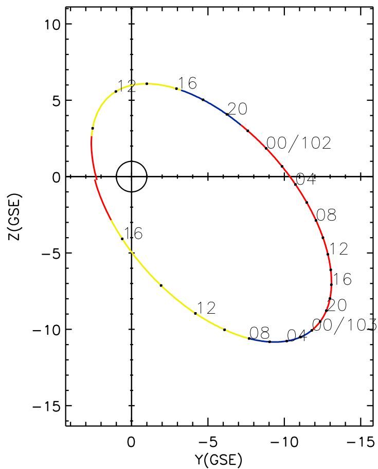
CLUSTER 2 orbit 2005 101 (04/11) 08:35 UT to 2005 103 (04/13) 17:40 UT
