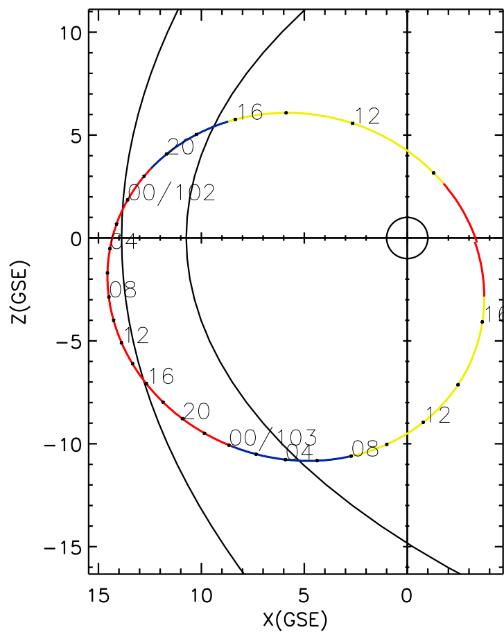
CLUSTER 2 orbit 2005 101 (04/11) 08:35 UT to 2005 103 (04/13) 17:40 UT
