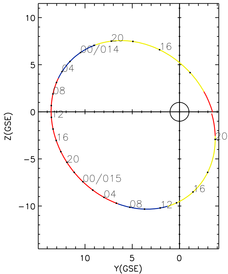
CLUSTER 2 orbit 2005 013 (01/13) 12:05 UT to 2005 015 (01/15) 21:10 UT
