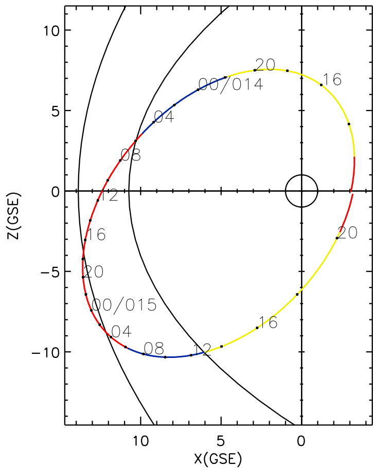
CLUSTER 2 orbit 2005 013 (01/13) 12:05 UT to 2005 015 (01/15) 21:10 UT
