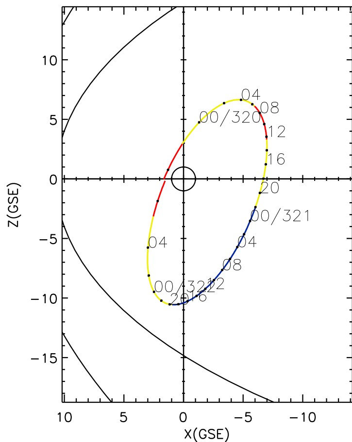
CLUSTER 2 orbit 2004 319 (11/14) 21:41 UT to 2004 322 (11/17) 06:41 UT
