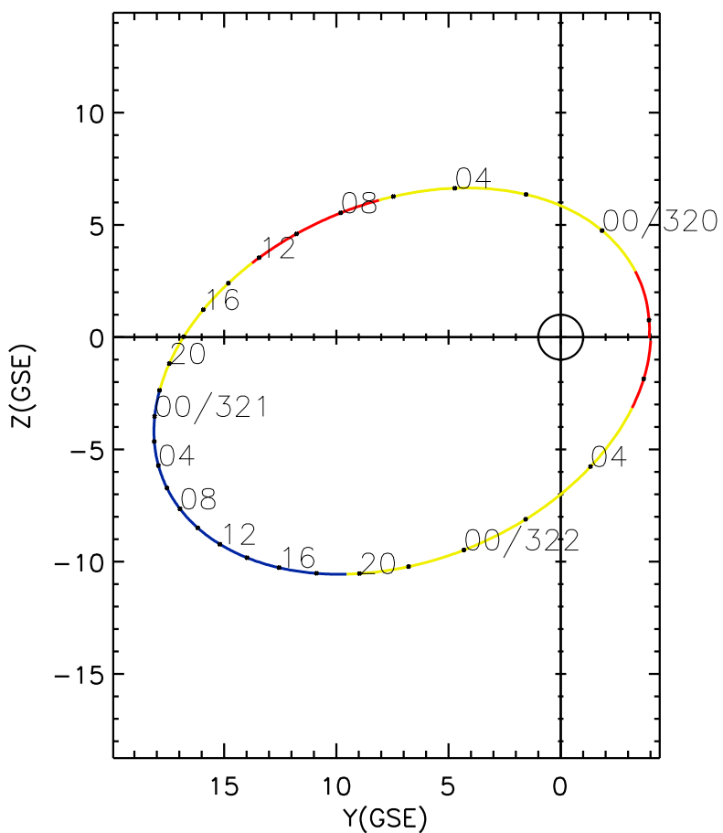
CLUSTER 2 orbit 2004 319 (11/14) 21:41 UT to 2004 322 (11/17) 06:41 UT
