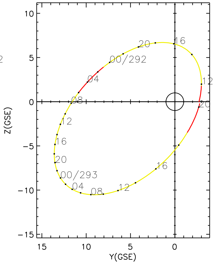
CLUSTER 2 orbit 2004 291 (10/17) 11:10 UT to 2004 293 (10/19) 20:10 UT
