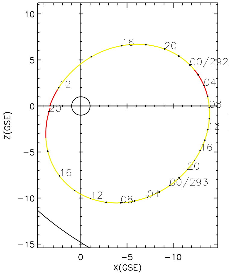
CLUSTER 2 orbit 2004 291 (10/17) 11:10 UT to 2004 293 (10/19) 20:10 UT
