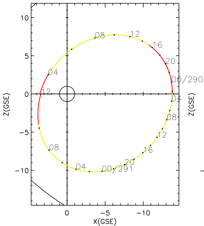
CLUSTER 2 orbit 2004 289 (10/15) 02:56 UT to 2004 291 (10/17) 12:01 UT
