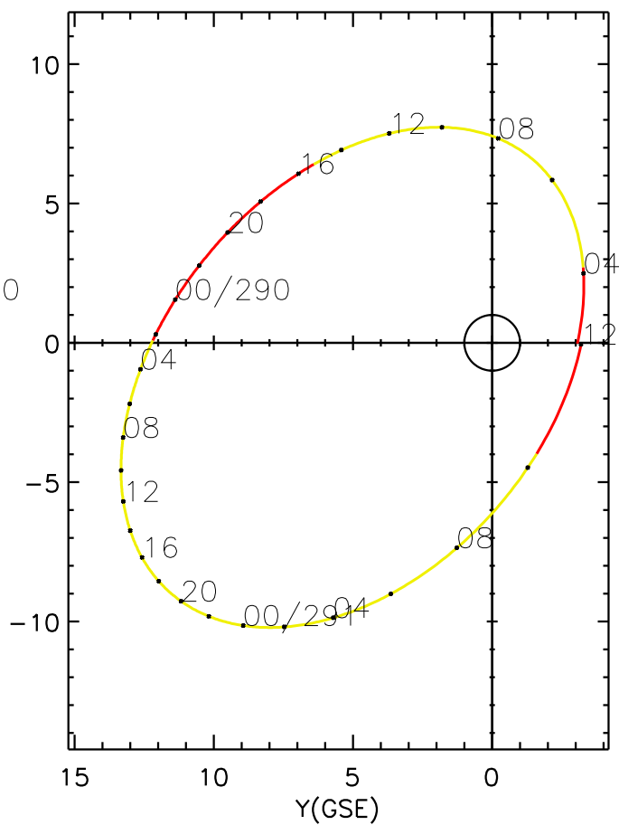
CLUSTER 2 orbit 2004 289 (10/15) 02:56 UT to 2004 291 (10/17) 12:01 UT
