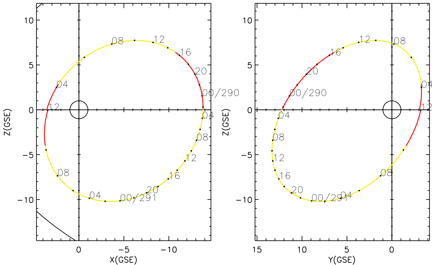
CLUSTER 2 orbit 2004 289 (10/15) 02:55 UT to 2004 291 (10/17) 12:00 UT
